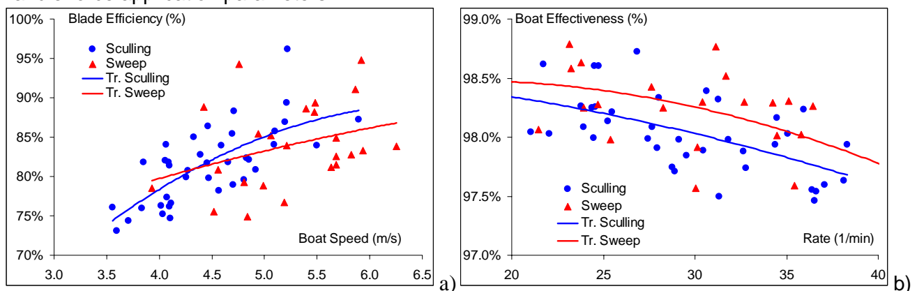
Figure 2. Dependencies of Blade Efficiency on Boat Velocity (a) and Boat Effectiveness on Stroke Rate (b)
